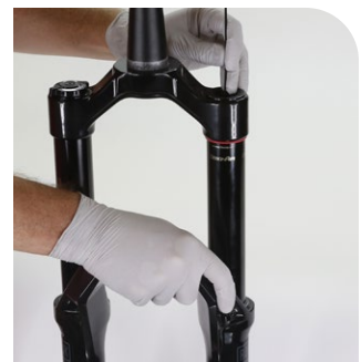
Pick or small hex wrench DebonAir+
